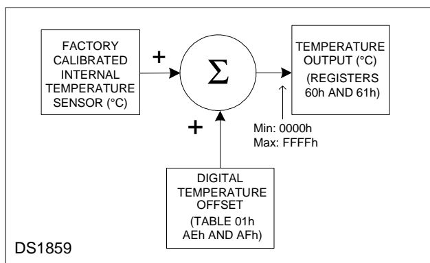
Figure 1. Digitally Applied Temperature Offset
